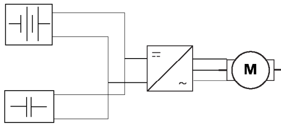
Figure 5. Passive BEV using a HESS topology
