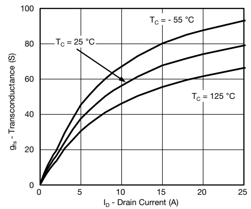
Transconductance
