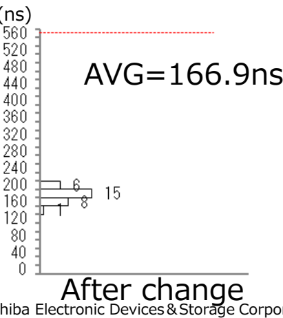
tDESAT(FAULT) (CDESAT=100pF, VCC1=5V, VCC2=30V, Rg=10Ω, RF=2.1kΩ)
