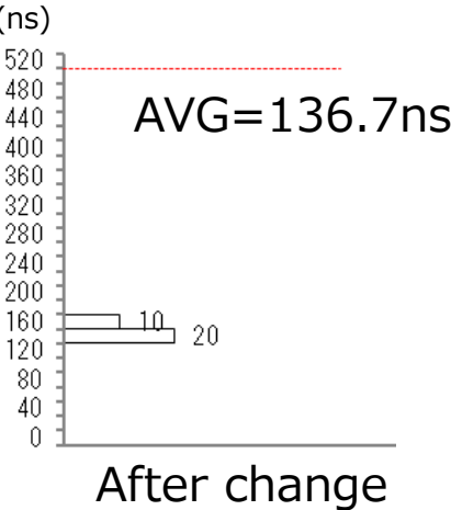
tDESAT90% (CDESAT=100pF, VCC1=5V, VCC2=30V, Rg=10Ω, RF=2.1kΩ, CG=25nF)
