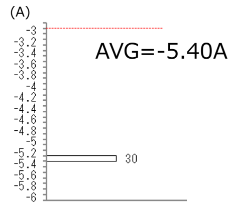
IOPH (VO=VCC2-7V, VCC2-VEE=15~30V)
