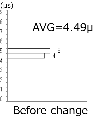
tDESAT10% (CDESAT=100pF, VCC1=5V, VCC2=30V, Rg=10Ω, RF=2.1kΩ, CG=25nF)
