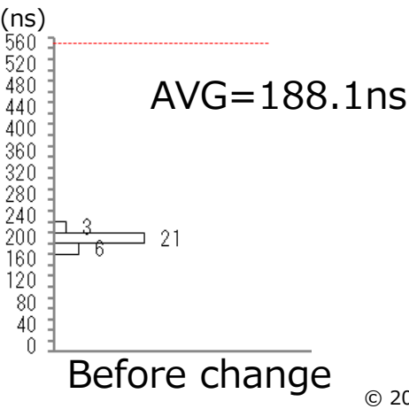
tDESAT(FAULT) (CDESAT=100pF, VCC1=5V, VCC2=30V, Rg=10Ω, RF=2.1kΩ)
