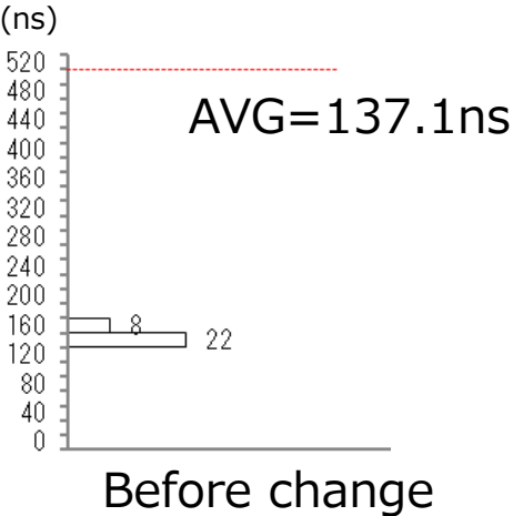
tDESAT90% (CDESAT=100pF, VCC1=5V, VCC2=30V, Rg=10Ω, RF=2.1kΩ, CG=25nF)
