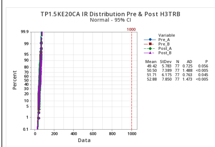
TP1.5KE20CA IR Distribution Pre & Post H3TRB
