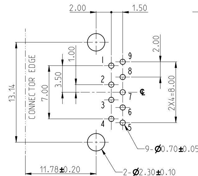
RECOMMENDED PCB LAYOUT-TOP VIEW (OTHER GENERAL TOLERANCES: ±0.05)
