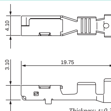
Female Terminal
