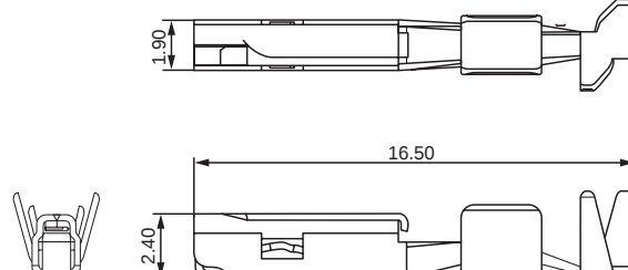
Female Terminal
