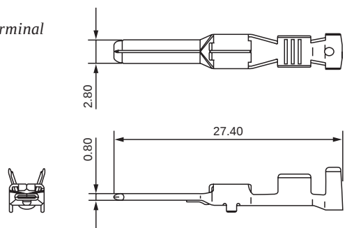
Female Terminal
