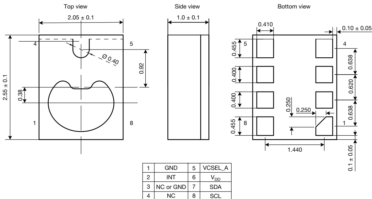
Fig. 12 - VCNL36826S Package Dimensions
