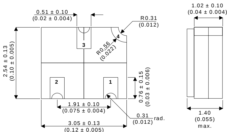
LCC1-4 (Underside View)
