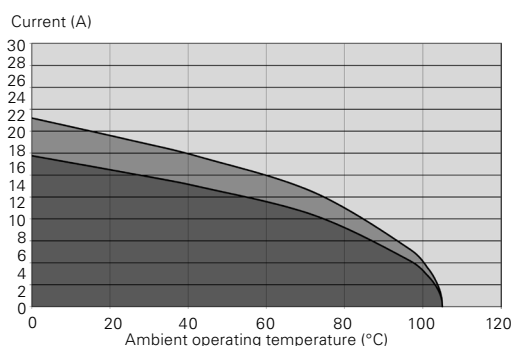
Fig.2: UTGX 12-8 – Wire section 16 AWG
