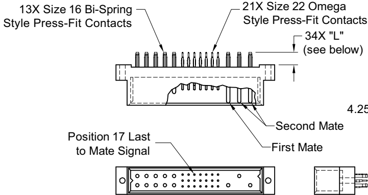
CONNECTOR DIMENSIONS
