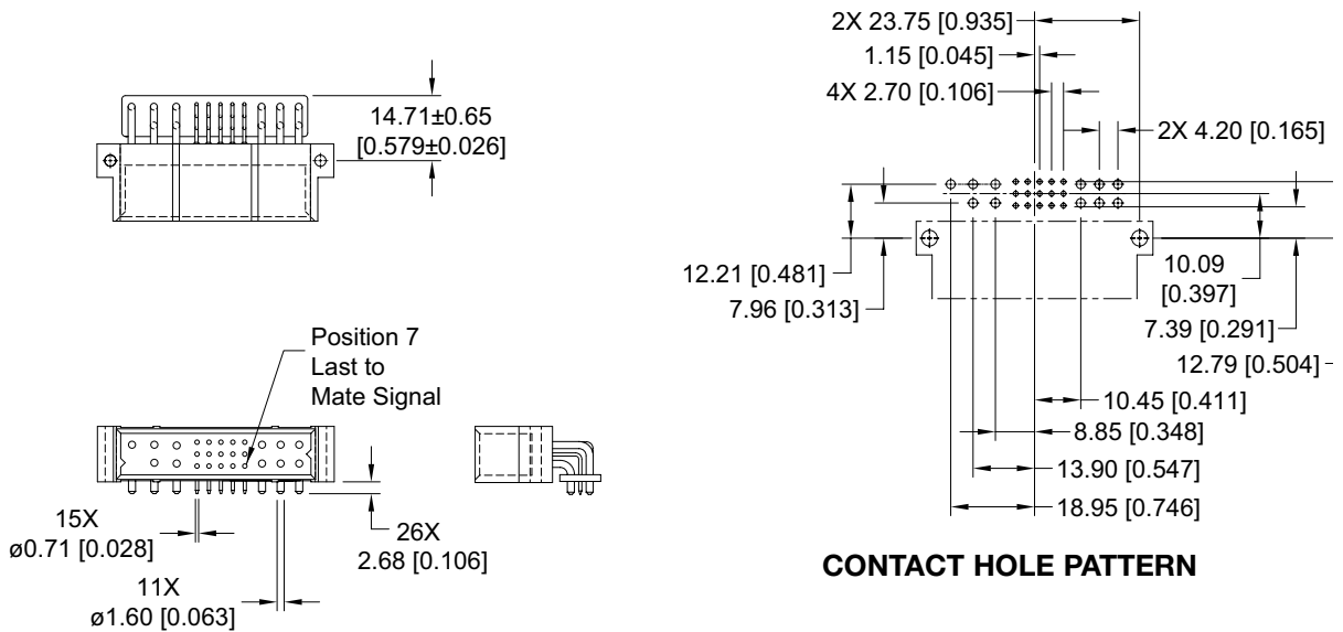
CONNECTOR DIMENSIONS
