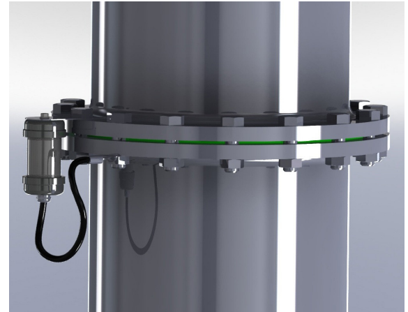
Figure 10 100 kA SPD for use on isolated flange ROW applications
