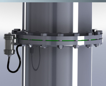
Figure 6 Isolated flange spark gap protection scheme
