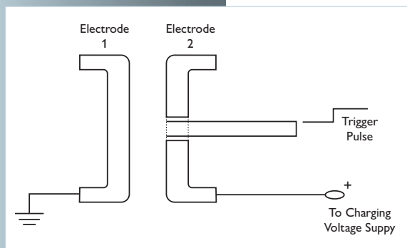
Figure 5 Triggered spark gap
