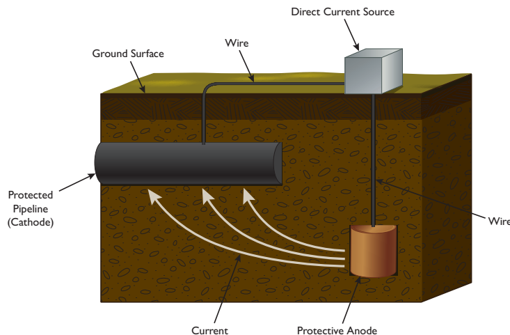
Figure 3 Impressed Current System
