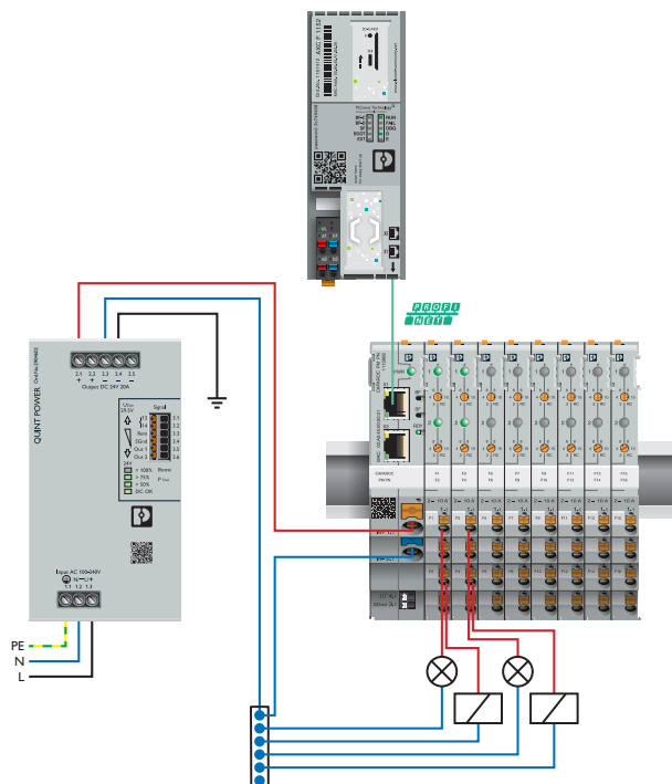
Application drawing
