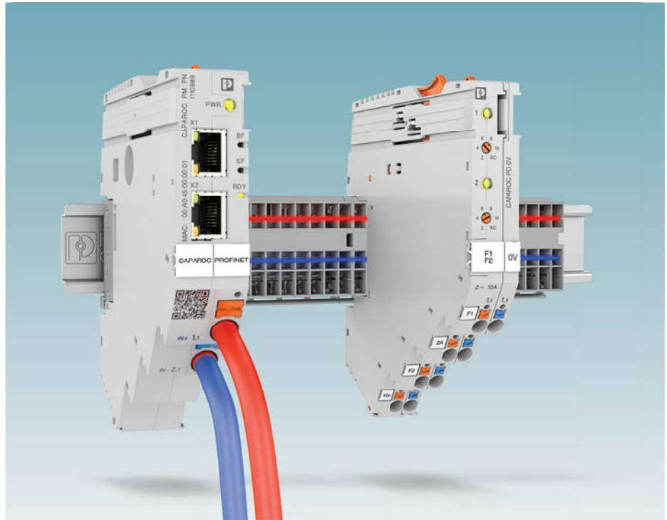
Power distribution via the current rails
