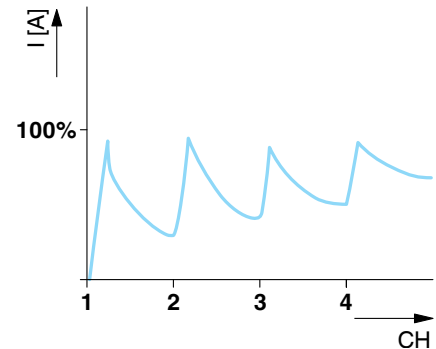
Cascaded connection of four channels
