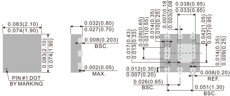
DFN2020-8L
