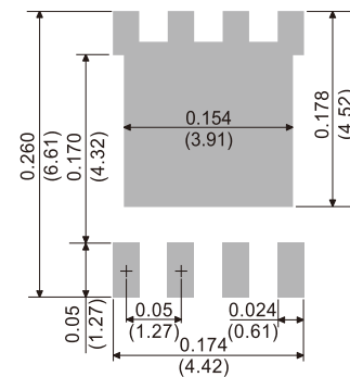
DFN5060B-8L
