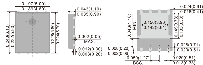
DFN5060B-8L
