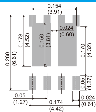
DFN5060B-8L
