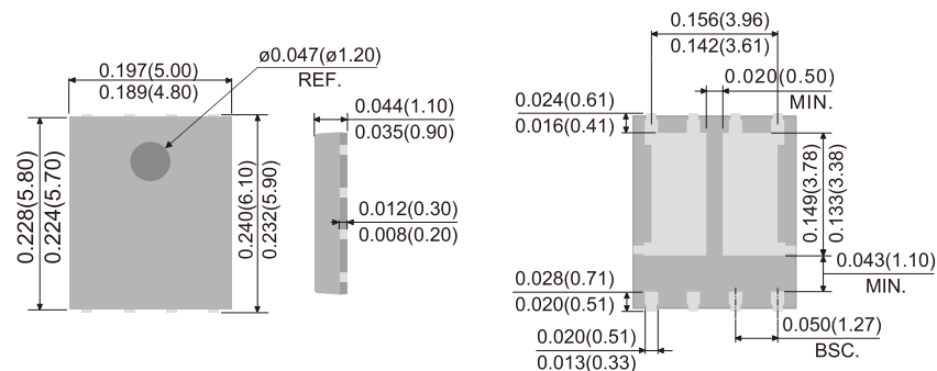
DFN5060B-8L
