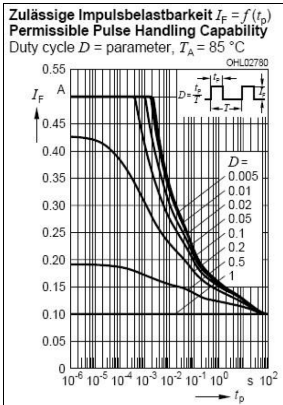
Figure 8: Example of pulse current specifications for PWM driving at T_A=85^\circ\text{C}
