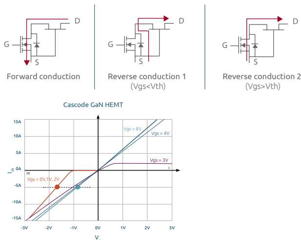
Figure 4 GaN FET operation
