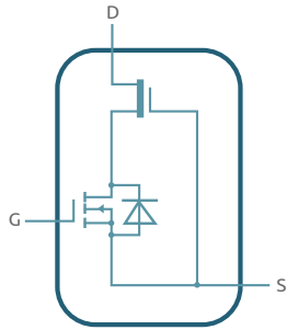
Figure 2 Cascode schematic
