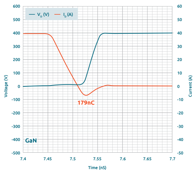
GAN041-650WSA Reverse turn-off, 41mΩ 400V, 40A, 800A/μs, Q_{rr} =179nC
