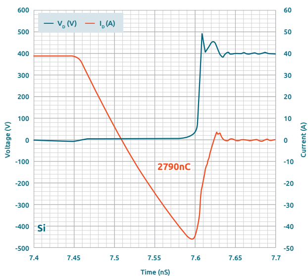
Si MOSFET Reverse turn-off, 41mΩ 400V, 40A, 800A/μs, Q_{rr} =2790nC
