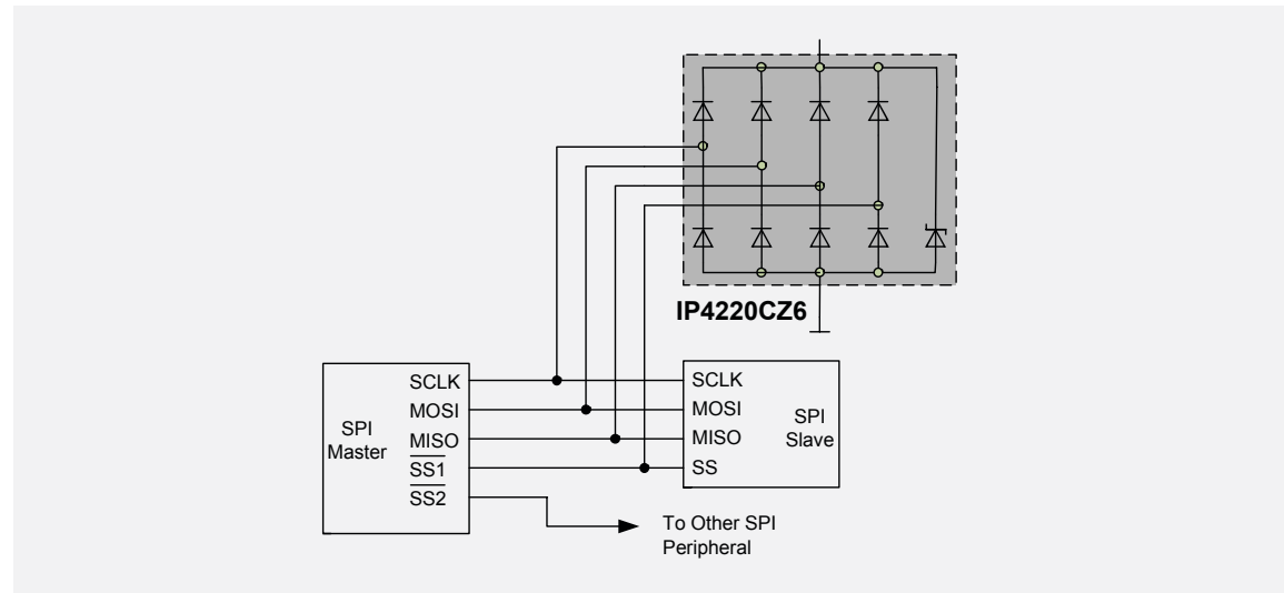
SPI protection showing a single device with a four-line, rail-to-rail diode
