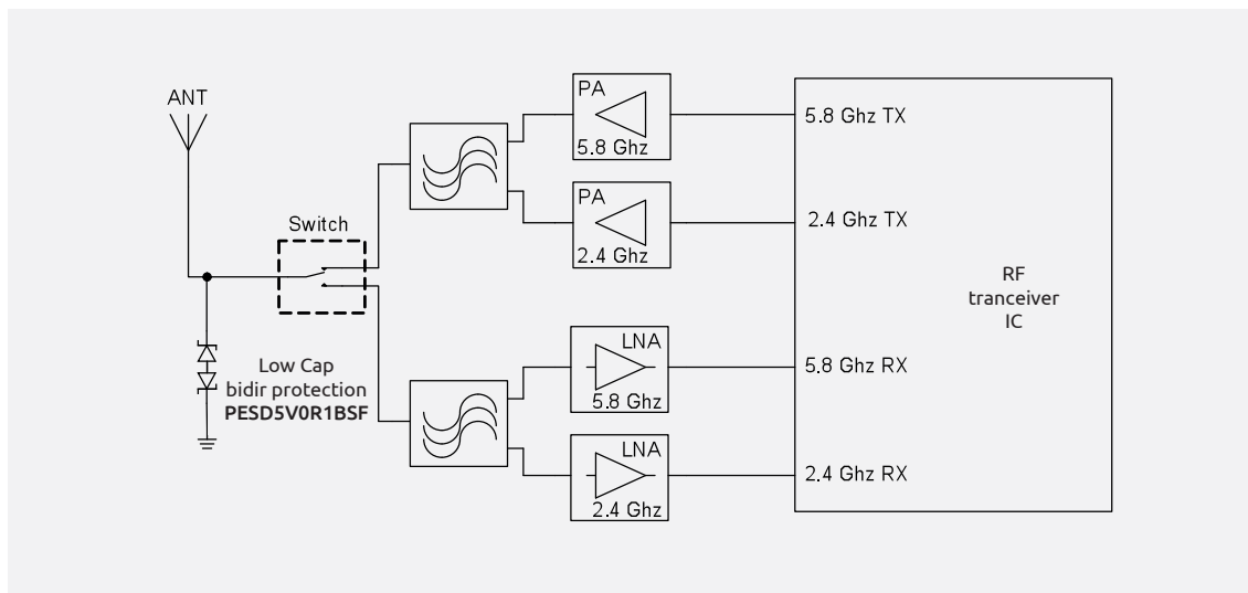
Dual-band WLAN ESD protection using PESD5V0R1BSF
