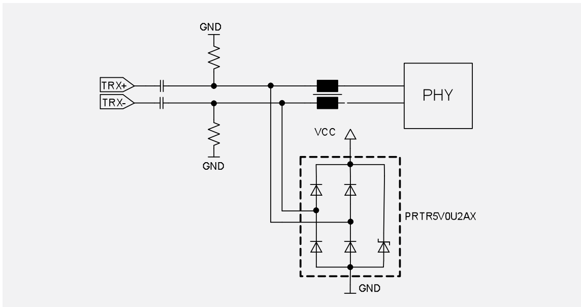
BroadR-reach protection, single channel
