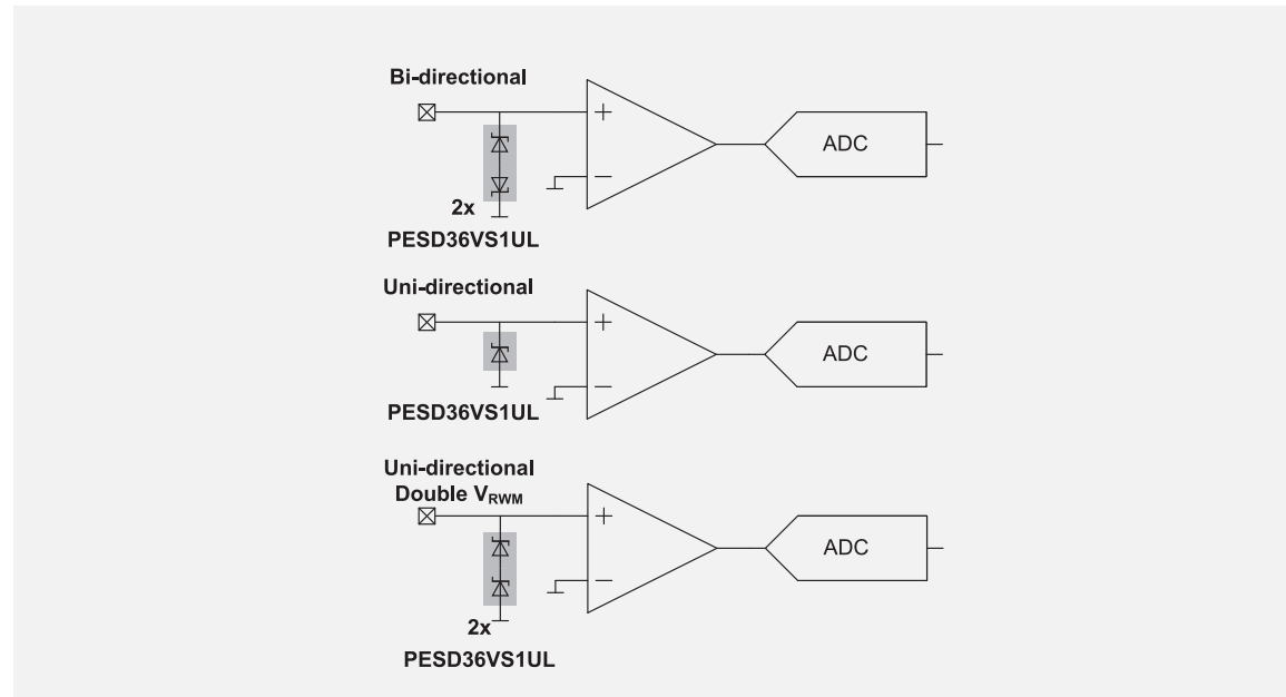
Analog I/O protection using the PESD36VS1UL with single or multiple devices
