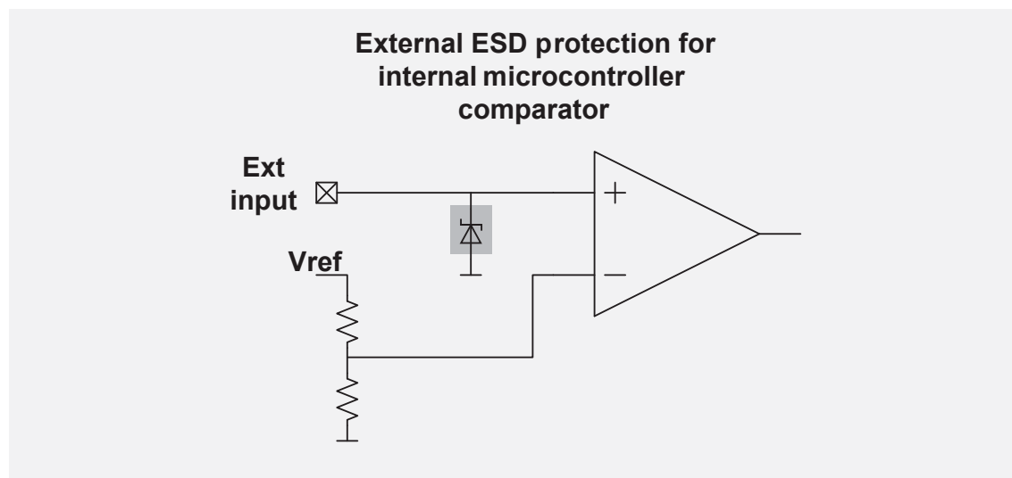
Unidirectional, low-voltage comparator ESD protection
