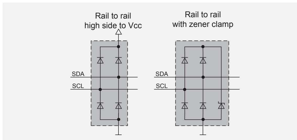
I 2 C protection two rail-to-rail configurations that minimize capacitive line loading
