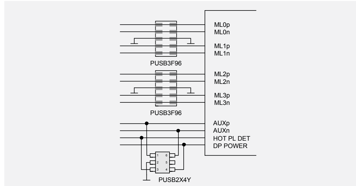
DisplayPort ESD protection with high-speed lines protected with PUSB3F96 and low-speed lines with PUSB2X4Y
