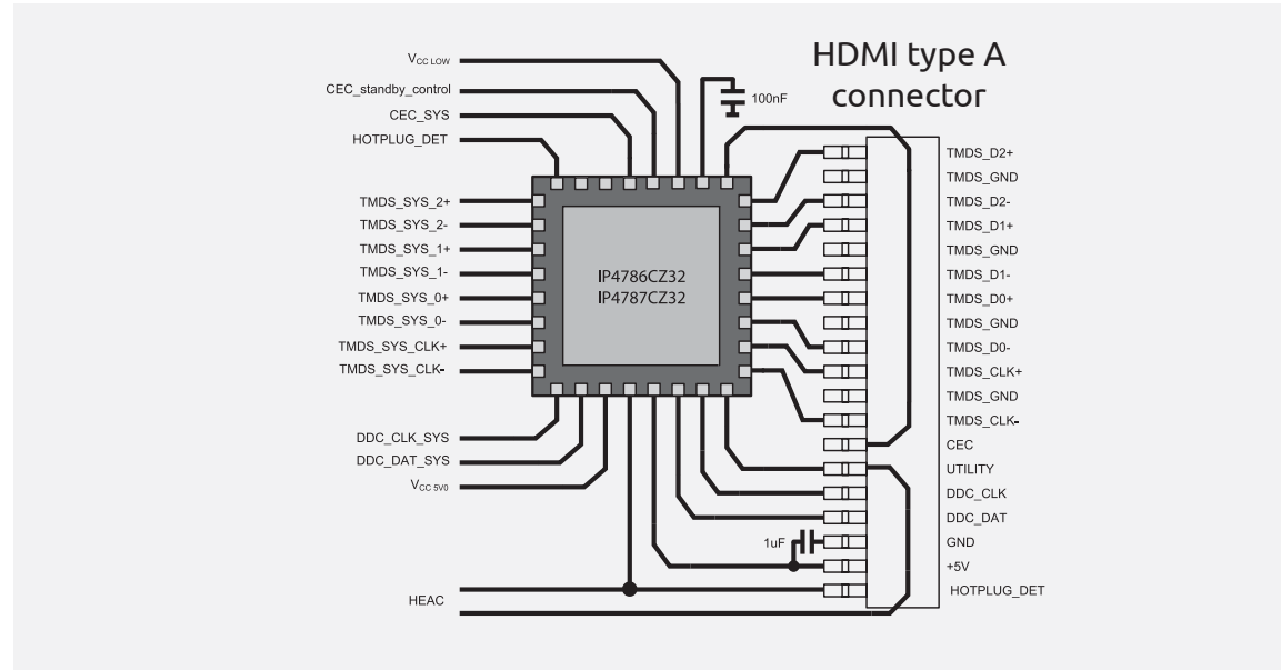
HDMI single-device ESD protection with level shift, showing IP4787CZ32 for receiver and IP4786CZ32 for transmitter applications.
