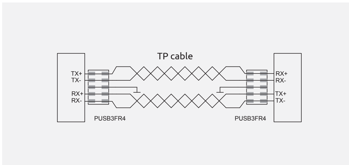
General high-speed differential mode signaling line ESD protection (actual data rate influences device choice)
