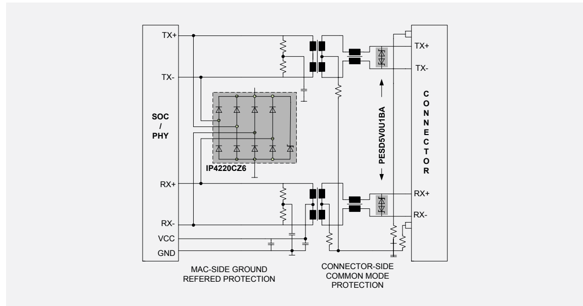
10/100 ESD protection, with ground-referred protection on the MAC side and Common mode protection on the connector side
