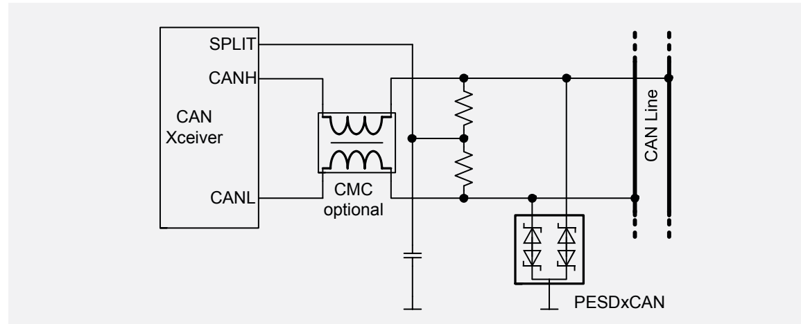
CAN system architecture with a single device to protect the CAN node
