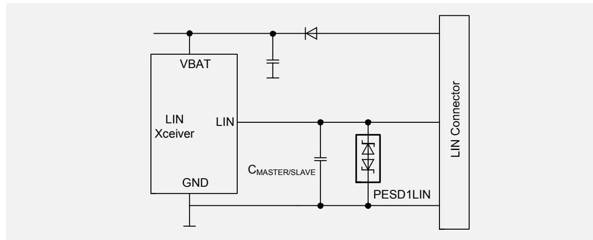
LIN system architecture with a single device to protect the LIN node
