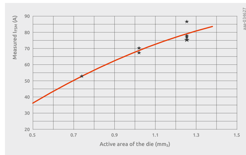
Figure 49 | I_{FSM} for a 5.5\text{ms} square wave pulse as a function of active chip area.
