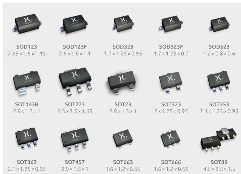
Figure 92 | Table of Nexperia diode leaded-packages with outline and dimensions in mm.
