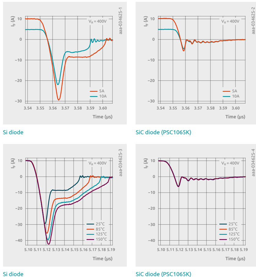
Figure 35 | Comparison of reverse recovery behavior of SiC vs. Si diodes.
