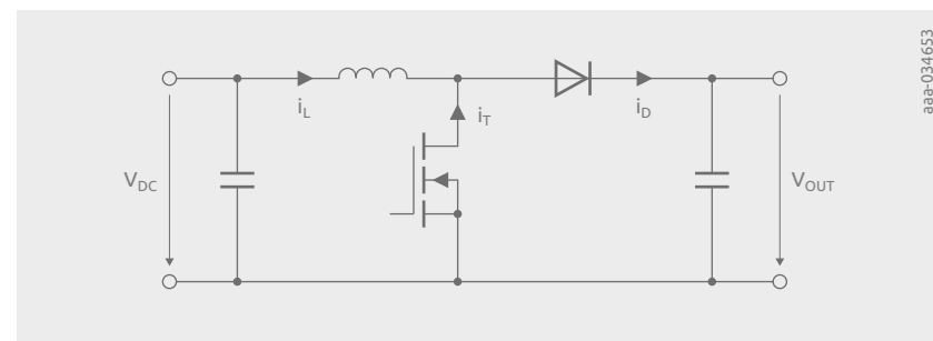
Figure 135 | Schematic of a boost converter
