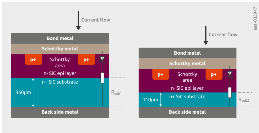
Figure 37 | Substrate resistance reduction through back-side grinding.
