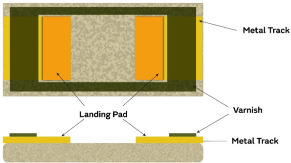
Figure 9: Example of NSMD designs with 2 pads.
