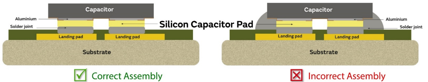
Figure 3: NSMD Assembly
