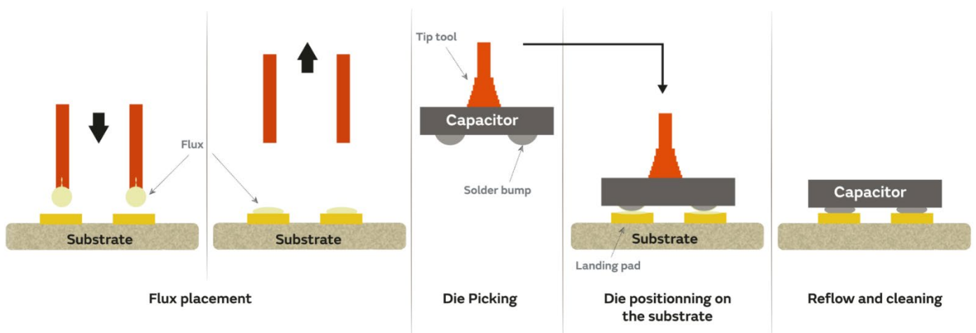
Figure 11: Assembly process by flux stamping on bumped capacitor with SAC305 terminations
