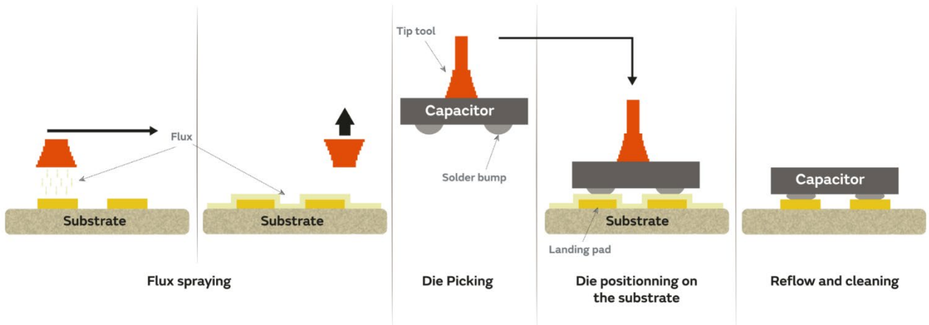
Figure 12: Assembly process by flux spraying on bunched capacitors with SAC305 terminations
