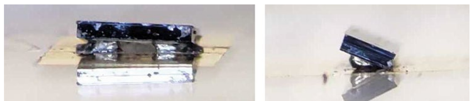
Figure 5 : Si-cap tilting examples, please note the solder excess
