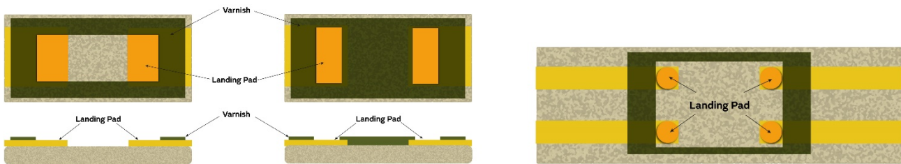
Figure 7: Examples of SMD designs, 2 pads on the left, 4 pads on the right
