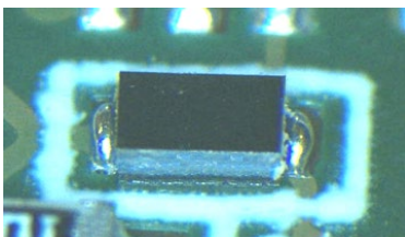
Figure 4 : Example of mis-assembly due to solder paste excess
