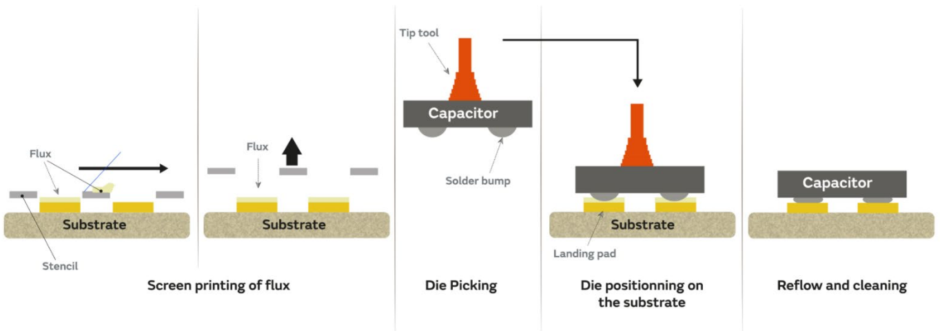
Figure 13: Assembly process by screen printing of flux on bunched capacitors with SAC305 terminations
