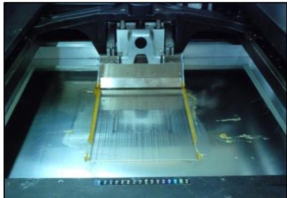
Flux Printing / Ball Attach
