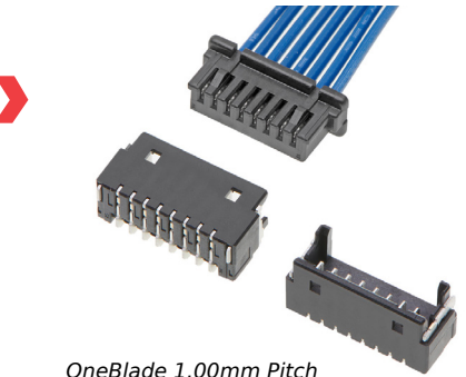
OneBlade 1.00mm Pitch Wire-to-Board Connector System
