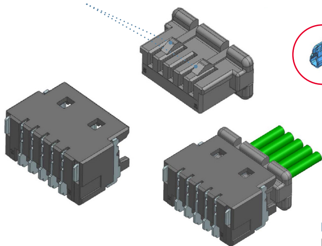
Receptacle Housing
