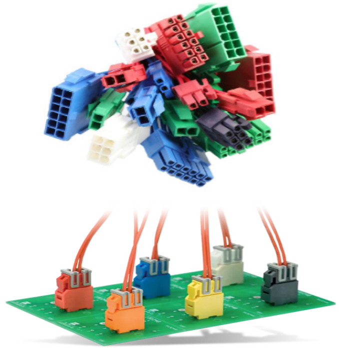
Figure 5: Color coding of connectors. Molex Mini-Fit Versa Color Power Connectors (top) and Molex CP-6.5 Series Wire to Board Connectors (bottom)
