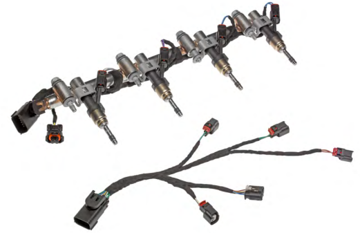
Custom Wire Harnesses for Vehicle Applications (V8 Fuel Rail Harness)
