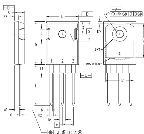
TO-247 Outline
