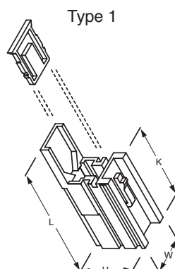
1 way housing for 8 mm receptacle (with secondary locking)
