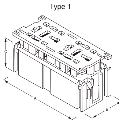
18 way / 2 relays housing
