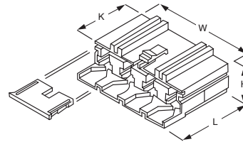
4 way housing for 8 mm receptacles ( with secondary locking )
