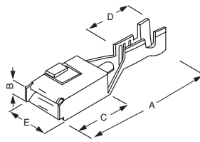
Micro-relay receptacles
