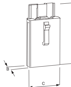
2 way housing for 2.8 mm receptacles
