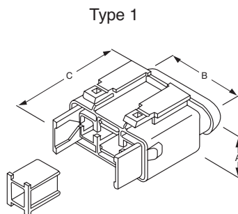
Housing for 8 mm Receptacle (with secondary locking)
