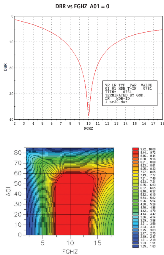
Figure 7. Tuned Frequency Q-Zorb at 0 degrees Angle of Incidence and at all angles. Red area shows best performance
