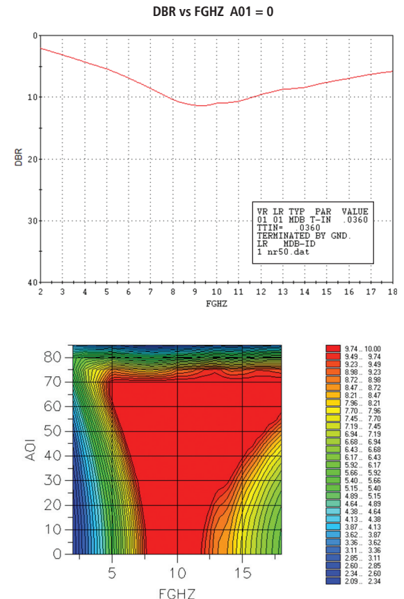
Figure 8. Surface Wave Q-Zorb; note broader area of highest absorption in red
