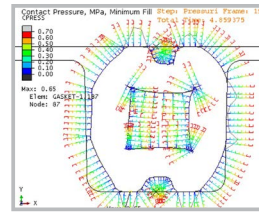
Contact pressure at minimum groove fill
