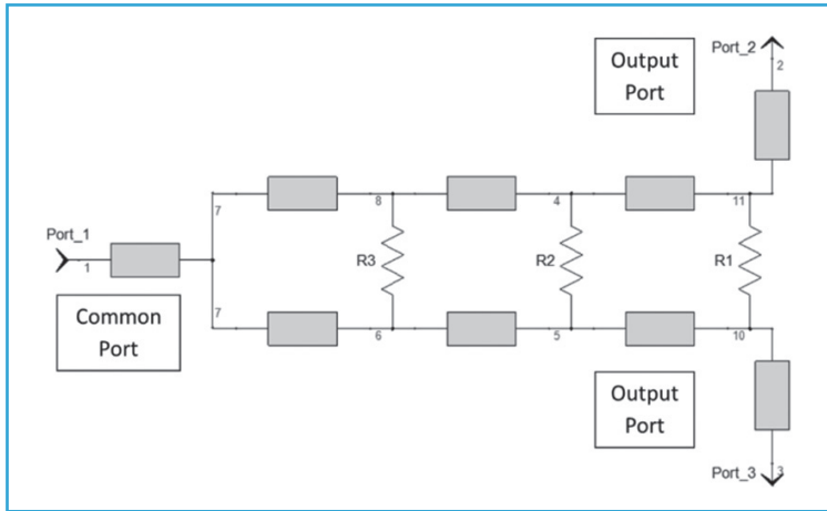
Figure 3: Multiple Section Wilkinson Power Divider
