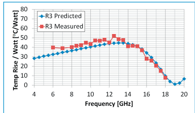
Figure 8: R3 Temperature Rise per Watt
