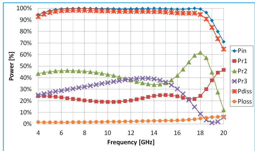
Figure 4: Power Budget for Odd Mode Excitation
