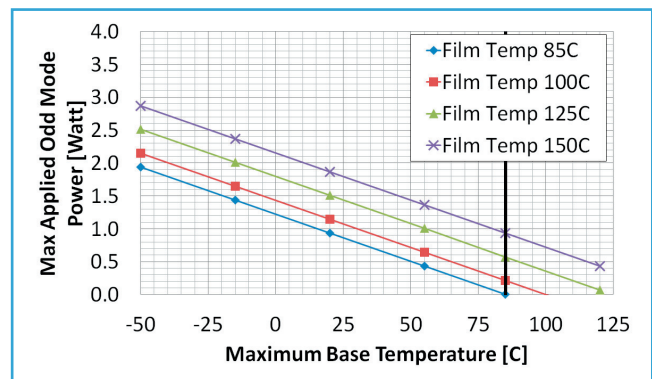
Figure 9: Maximum Dissipated Power vs Base Temperature vs Maximum Film Temperature at 18GHz
