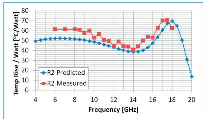
Figure 7: R2 Temperature Rise per Watt
