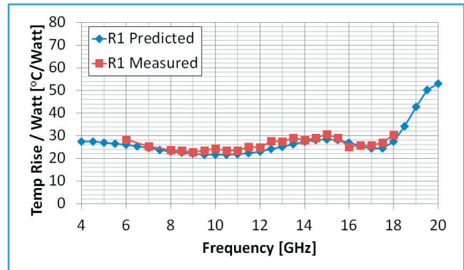
Figure 6: R1 Temperature Rise per Watt
