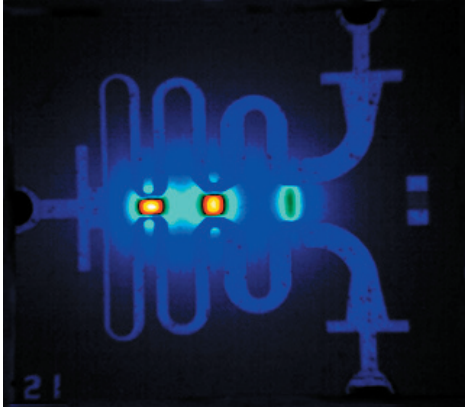
Figure 5: Thermal Image with 1Watt Applied in Odd Mode
