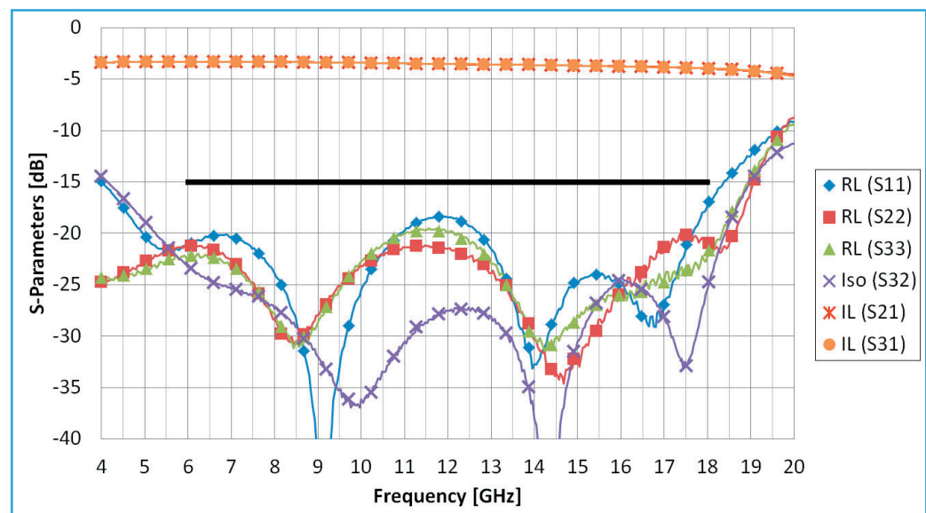
Figure 2: Measured performance of DLI PDW05758 Power Divider
