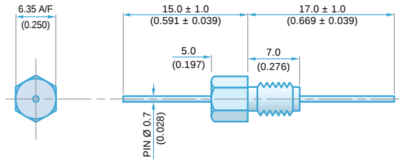
12-32 UNEF Class 2A Thread 6.35mm Hexagonal Head
