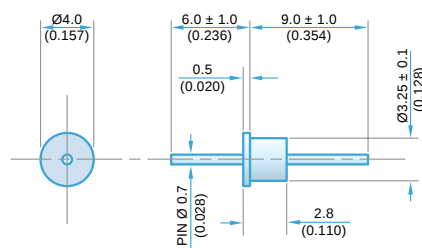
3.25mm Body Diameter Epoxy Sealed
