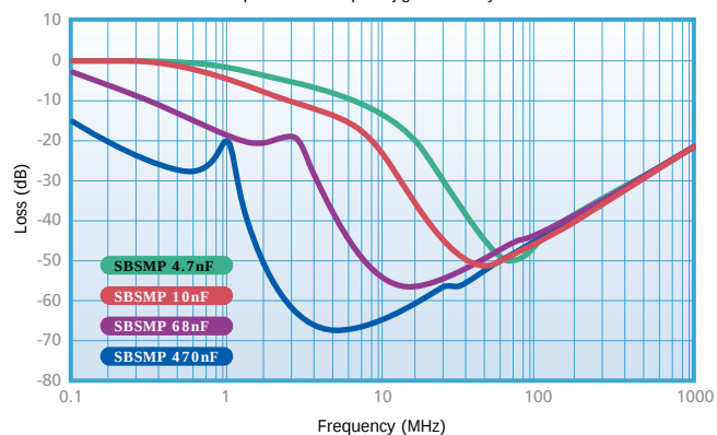
SBSMP Insertion Loss Open Board Stripline jig. 50ohm System
