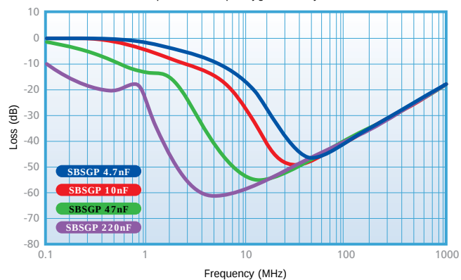
SBSGP Insertion Loss Open Board Stripline jig. 50ohm System
