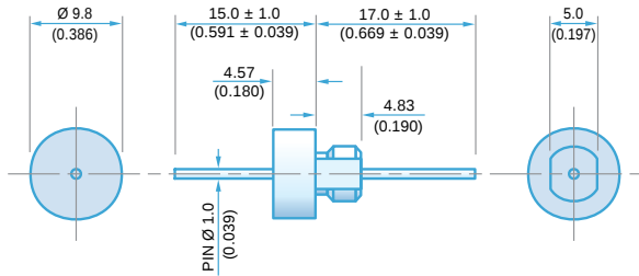
M6 x 0.75 - 6g Thread 9.8mm Round Head
