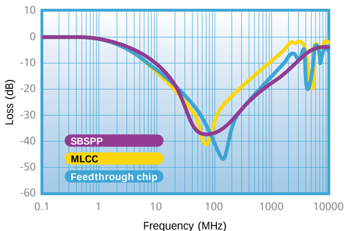
Comparison of 3.3nF SM filter types
