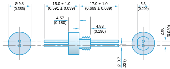
¼ -28 UNF Thread Class 2A thread Balanced Line EMI Filter Range
