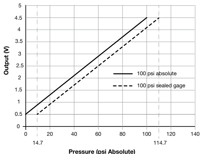
Figure 3. Absolute vs Sealed Gage Pressure vs Output
