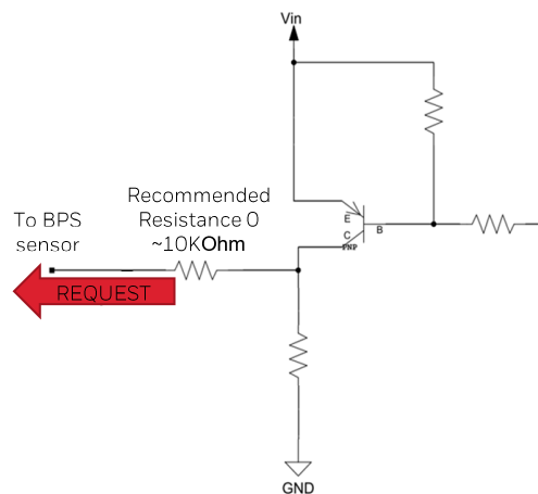
Figure 5. Recommended REQUEST pin BMS interface circuit
