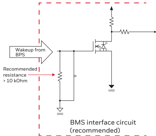
Figure 6. Recommended WAKEUP pin interface circuit
