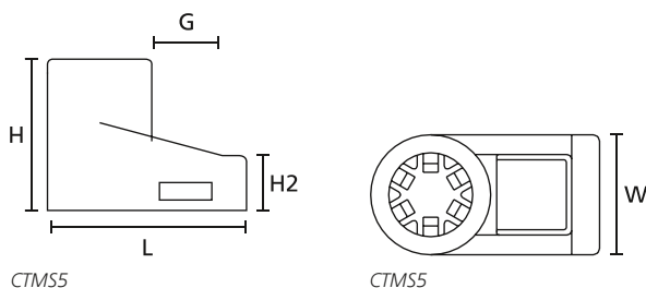
Fixing Element CTMS5 allows bundles to be routed alongside the stud.
