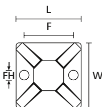
Cable Tie Mounts MB3, MB4, MB5 (plan view)
