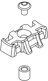
Suitable for welding studs (M8 internal bore & outer diameter 15 mm)
