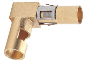
Figure 3: Solder contact example
