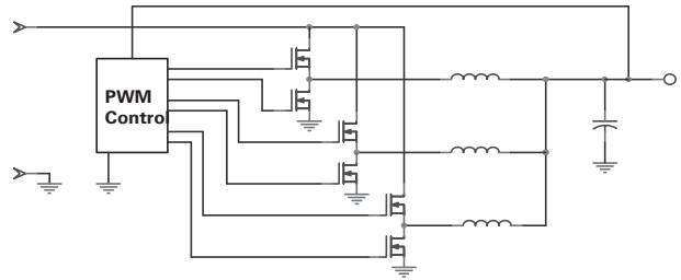
Figure 1. Multi-phase Voltage Regulator Module
