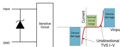
Figure 10: Overvoltage protection using a unidirectional TVS device.
