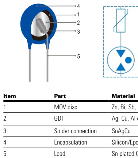
Figure 1: A typical MOVGT
