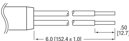
6" Wire Leads
