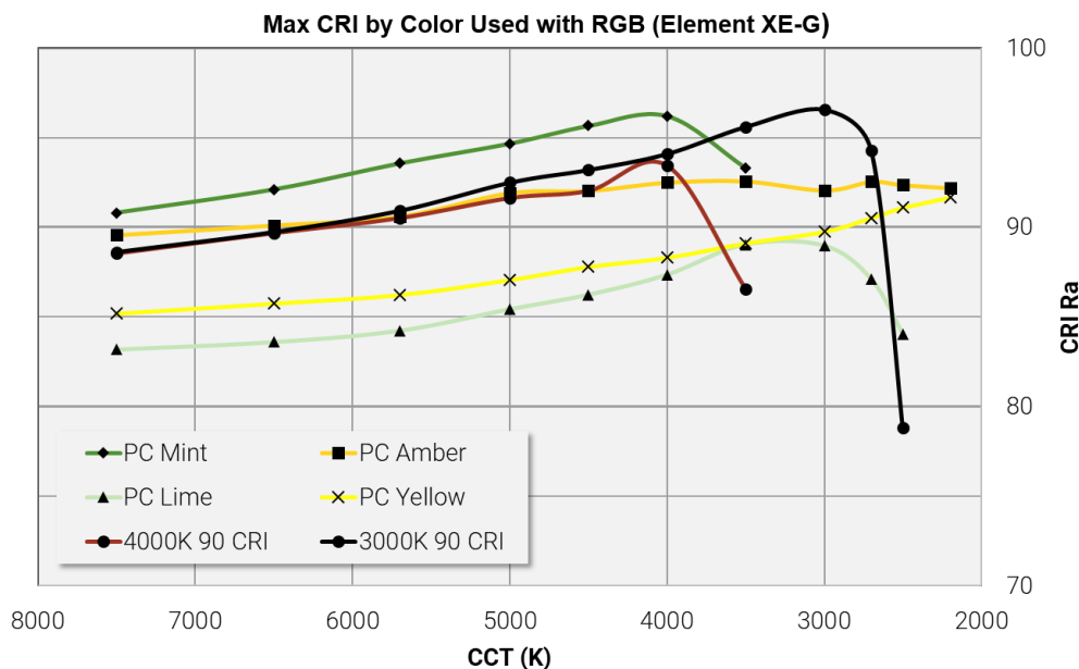
Figure 7: Maximum CRI achieved with each 4-channel configuration, sorted by the LED in the “white” position
