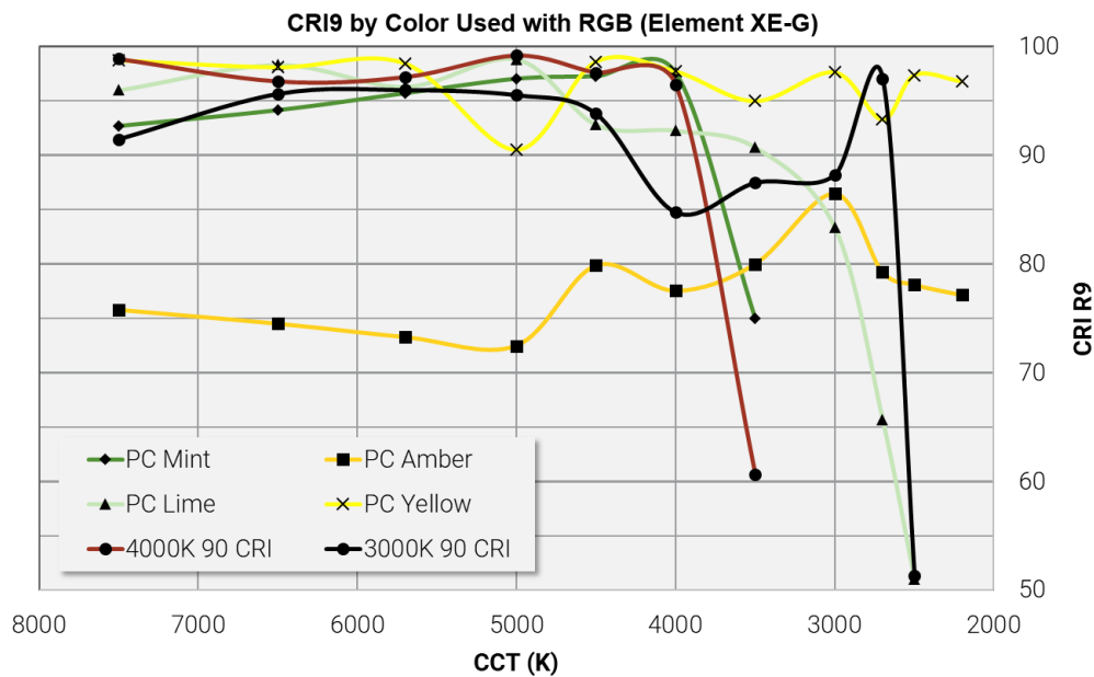
Figure 8: CRI R9 of each data point from Figure 7, sorted by the LED in the “white” position
