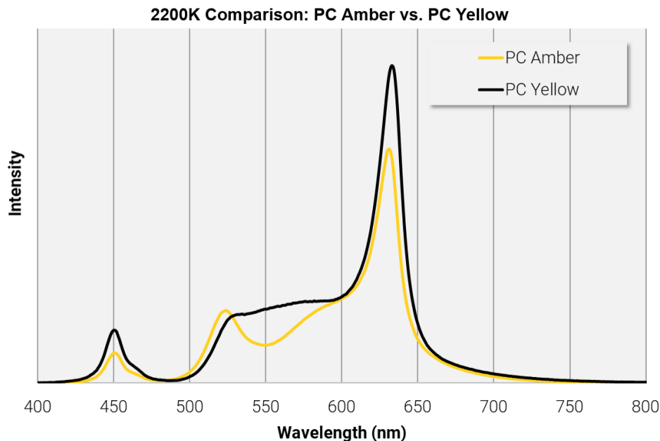
Figure 10: Raw spectral comparison of an RGB array with PC amber and PC yellow LEDs in the fourth position tuned to 2200 K. Both spectra were collected with a total input current of 3 A.
