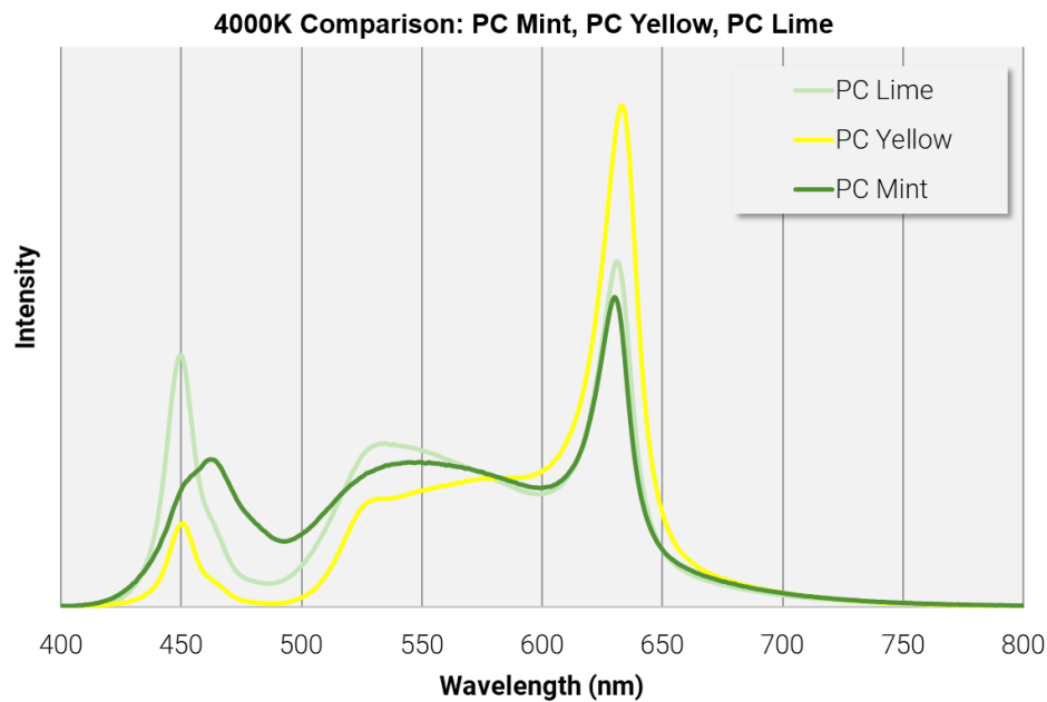
Figure 4: Spectral comparison at 4000 K of the three highest-lumen options that can be used with RGB in a 4-channel array
