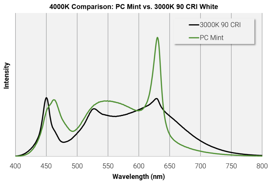
Figure 9: Raw spectral comparison of an RGB array with PC mint and with a 3000 K 90 CRI white LED in the fourth position tuned to 4000 K. Both spectra were collected with a total input current of 3 A.
