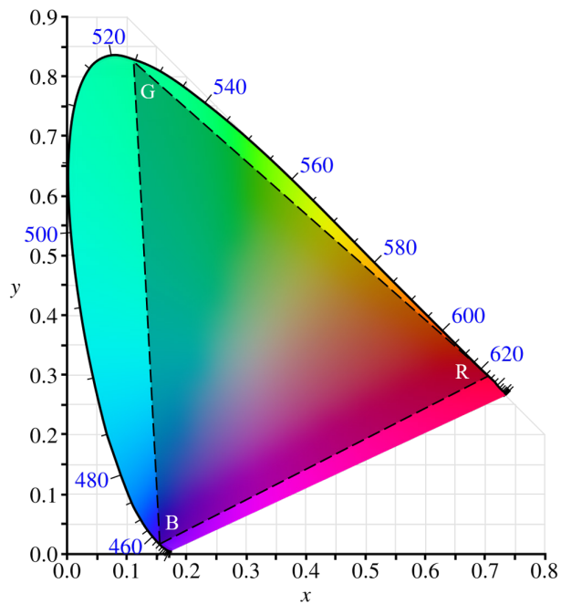
Figure 1: CIE color plot showing gamut triangle for RGB
