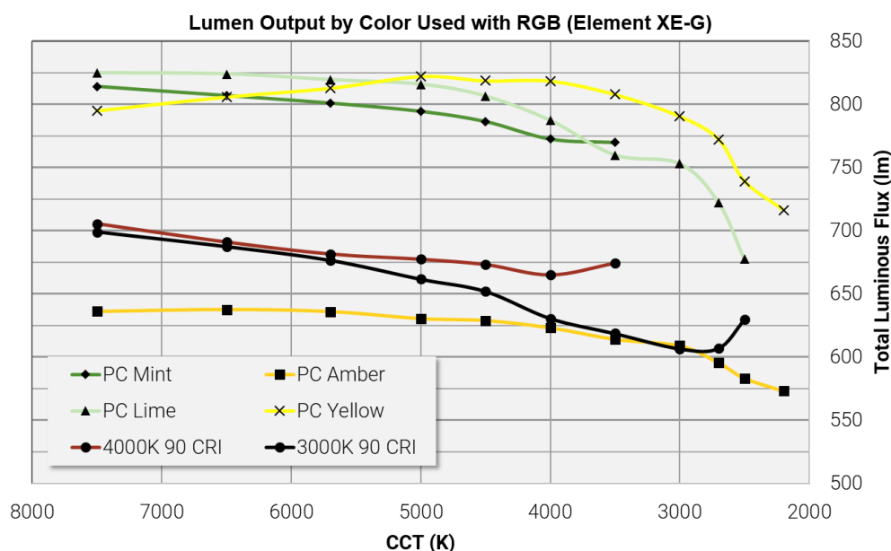
Figure 3: Luminous flux output of the 4-LED arrays sorted by the type of LED in the “white” position
