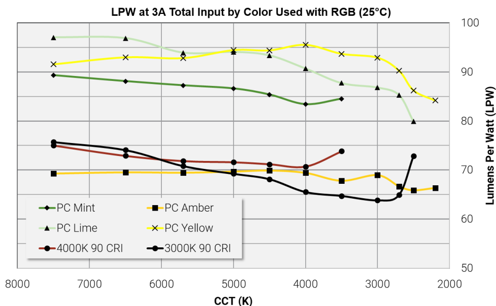
Figure 6: Luminous flux output of the 4-LED arrays, sorted by the type of LED in the “white” position
