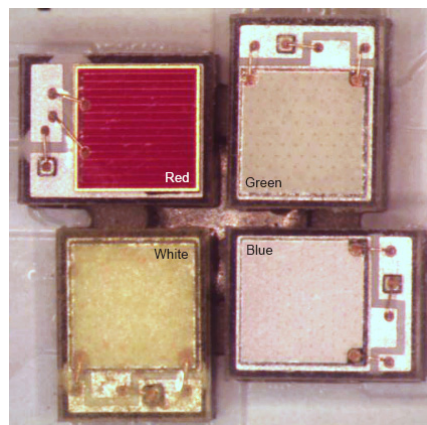
Figure 2: Four XLamp XE-G LEDs mounted on an MCPCB in a pinwheel configuration at approximately 200 \mu\text{m} edge-to-edge spacing
