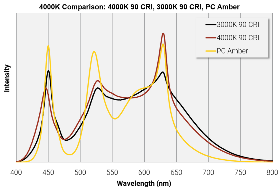
Figure 5: Spectral comparison at 4000 K of the three lower-lumen options that can be used with RGB in a 4-channel array. These options typically have a higher CRI than the “highest lumen” options in Figure 4.
