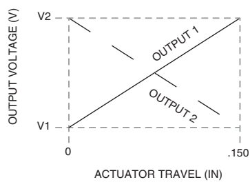
FIGURE 1: OUTPUT VOLTAGE
