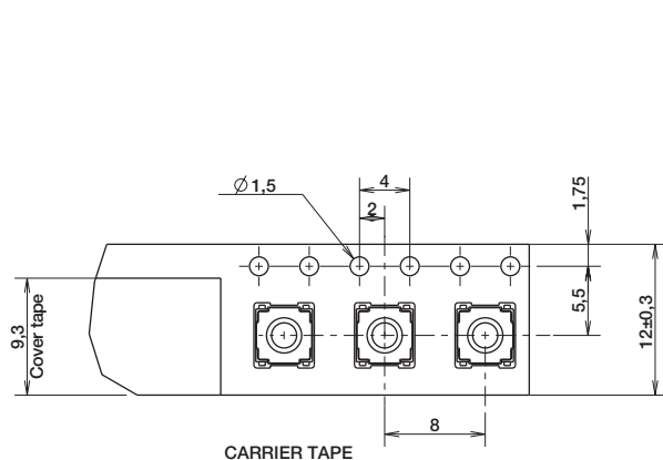
CARRIER TAPE
