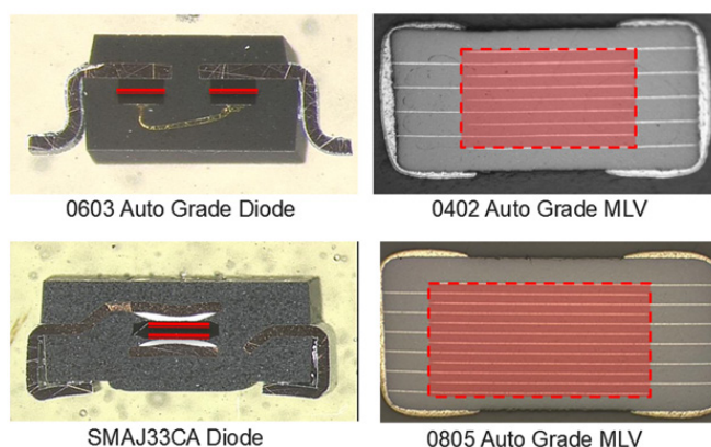
Figure 9. TVS Diode & MLV cross sections with active areas highlighted in red
