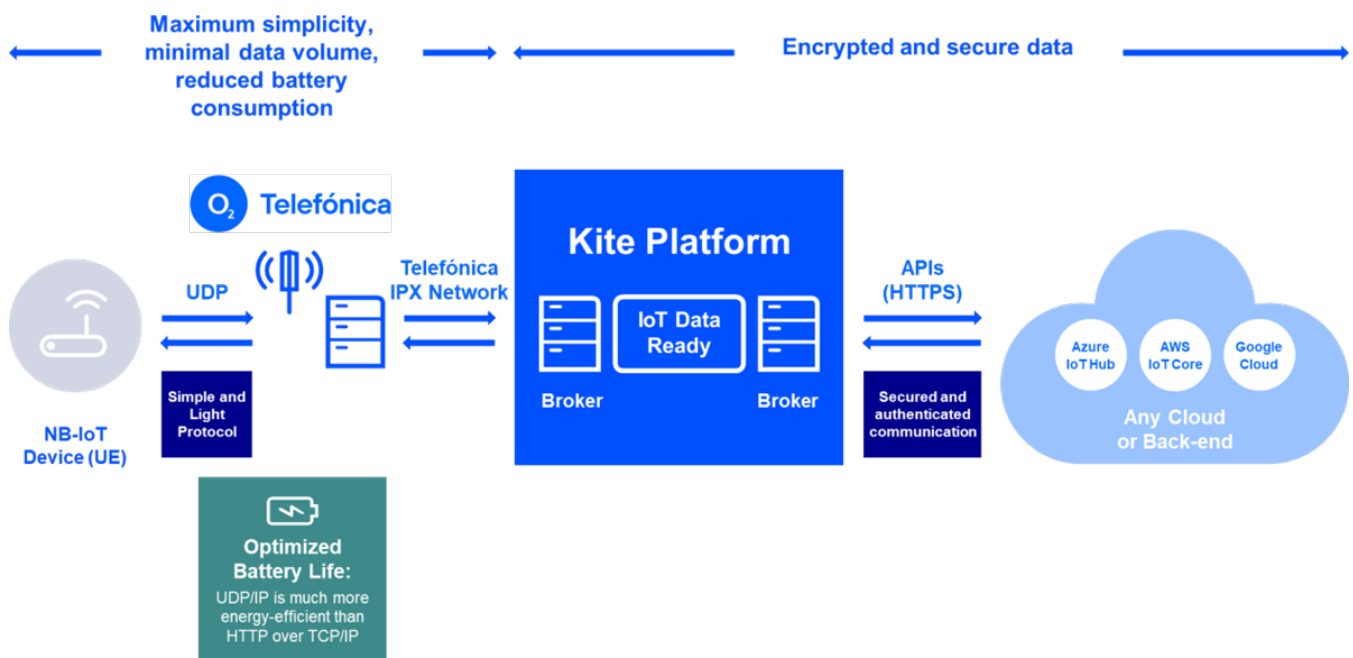
Figure 17: IoT Data Ready as broker service for battery-powered hybrid devices
