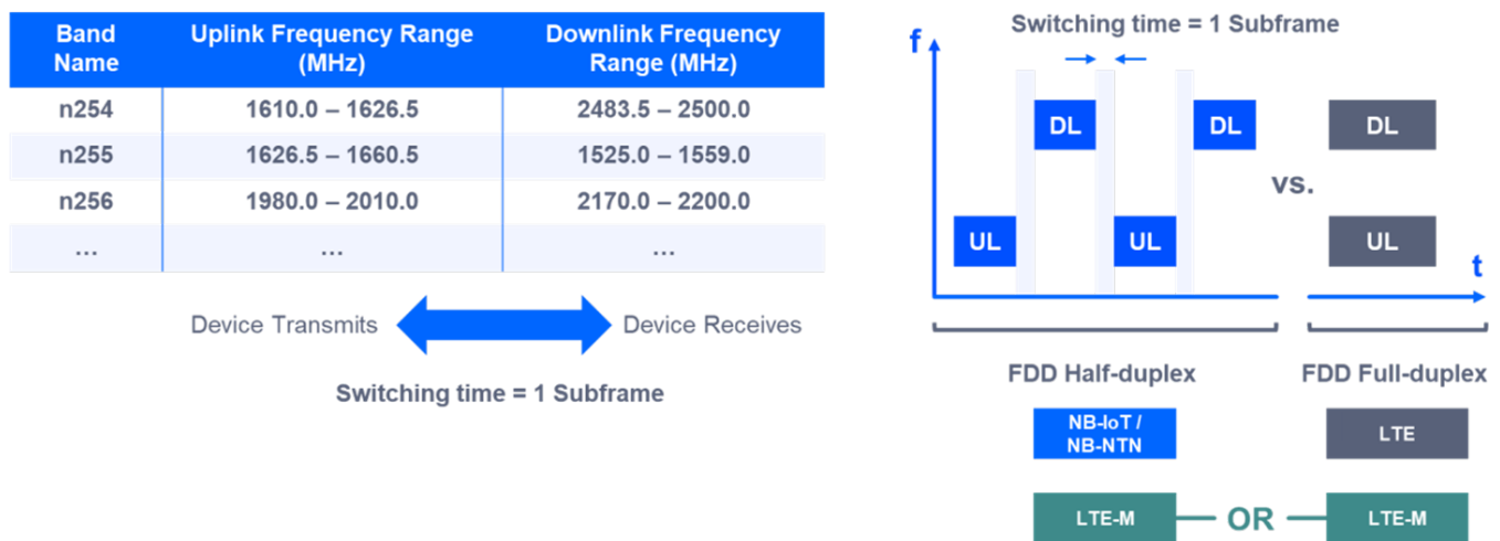
Figure 12: Frequency Division Duplex in NB-NTN
