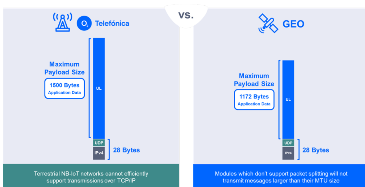
Figure 3: Comparison of Application Payload Sizes - Terrestrial NB-IoT vs. NB-NTN
