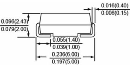
SMB/DO-214AA
