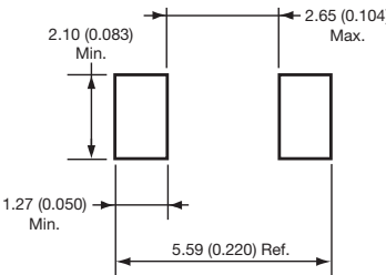
DO-214AA (SMB)
