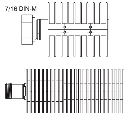
Model 3114N-F
