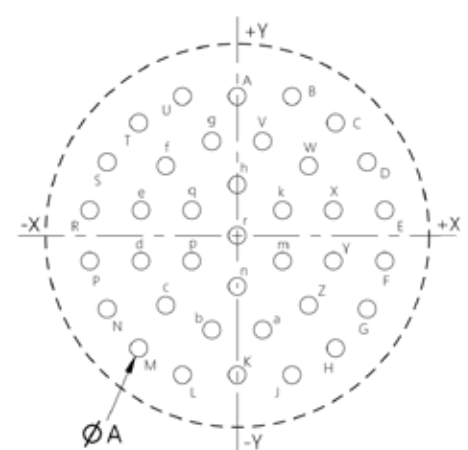
37 Contacts Size 16
