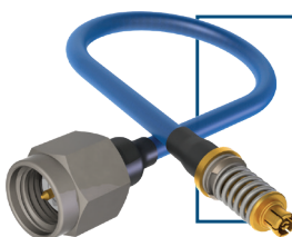
SMPM VITA to SMA Male Cable Assembly .085" Cable PN: 7032-6729-060 (6") PN: 7032-6729-120 (12")
