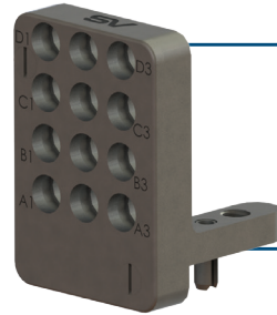
VITA 67.3 SMPS 12-Port Plug-In Connector Module SV PN: SF9311-60166
