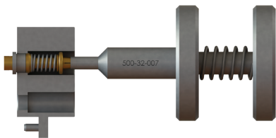
Figure 2.4 Adapter Removed From Contact Uses Tool PN 500-32-007
