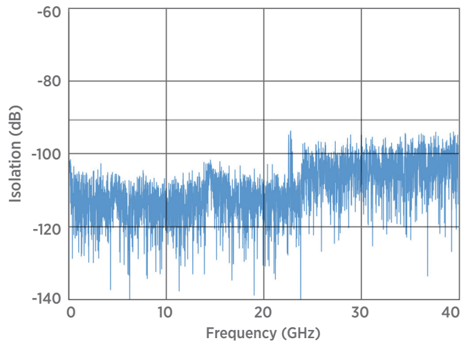
Figure 6.3 Electrical Isolation Plot (Mated Pair)
