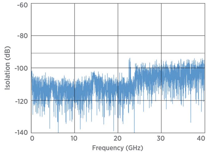
Figure 4.3 Electrical Isolation Plot (Mated Pair)
