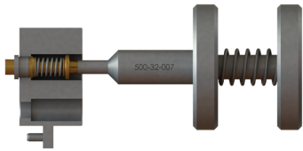
Figure 2.2 Adapter Fully Seated in Contact
