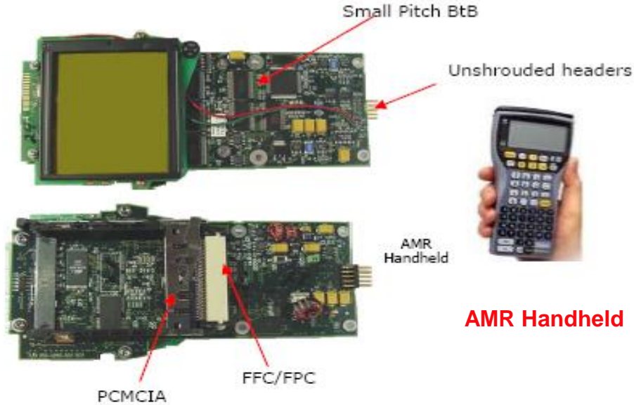
Unshrouded headers
