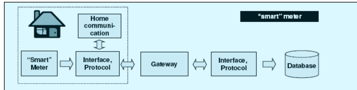
Smart Meter – Schematic Diagram
