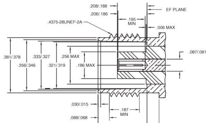
JACK
