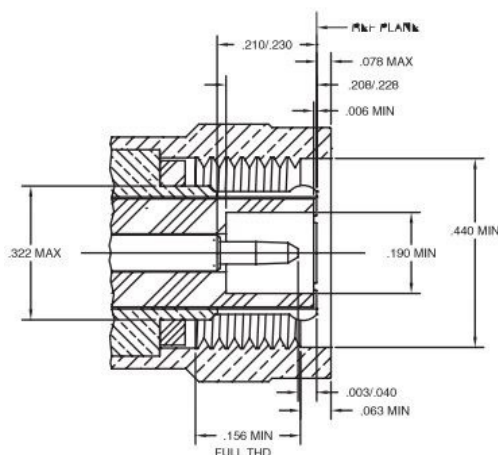
PLUG
