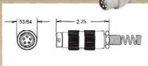
AJ-155 (M55116/11)
