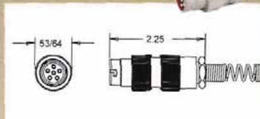
AJ-156 (M55116/12)
